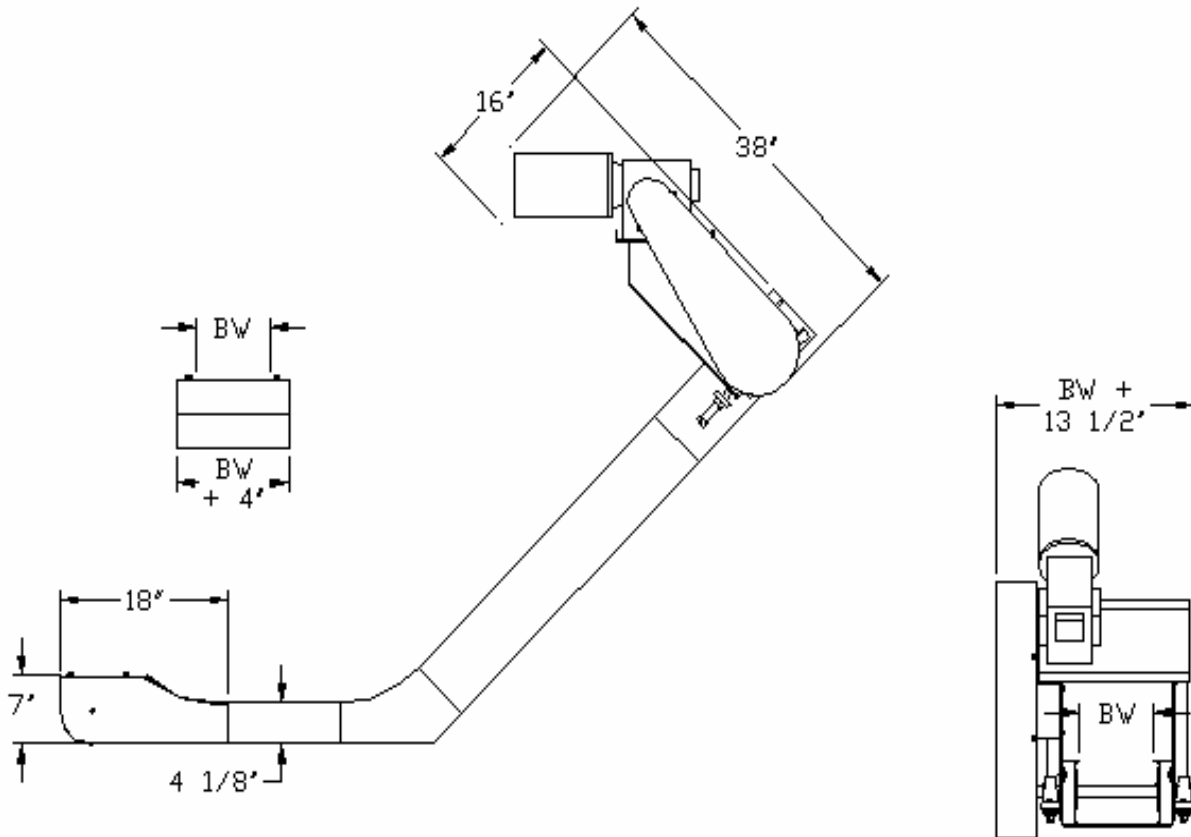
45° TOP MOUNT DRIVE
